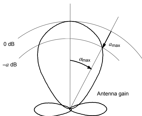
Figure H.2 – Calculation of the resulting gain reduction a
