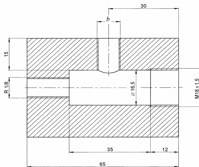
Figure F.3a – General view
