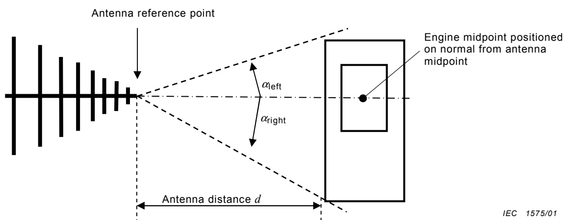
Figure H.1 – Determination of the maximum antenna angle
