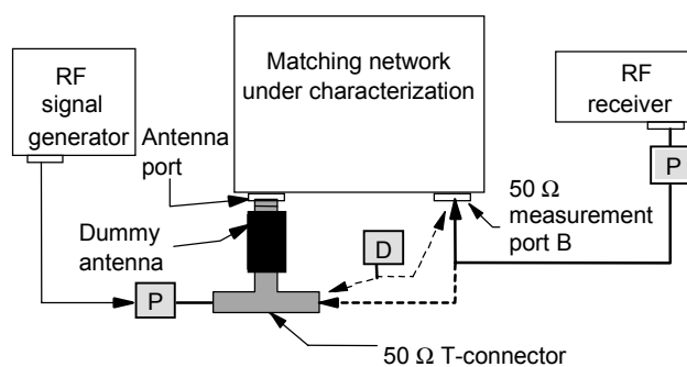
Figure B.2a – Method using network analyser
